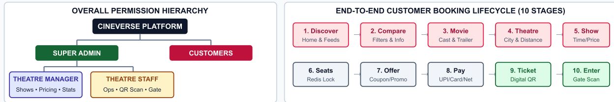
Figure 1.1: CineVerse Four-Role Governance Hierarchy & Ten-Stage Customer Booking Funnel
